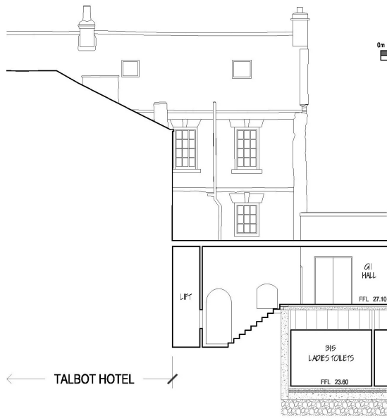
1 Section 34
