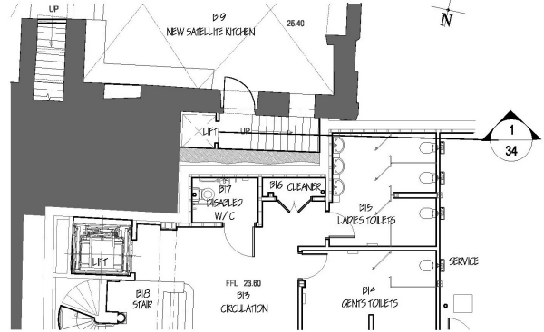
2 Basement Plan 34
